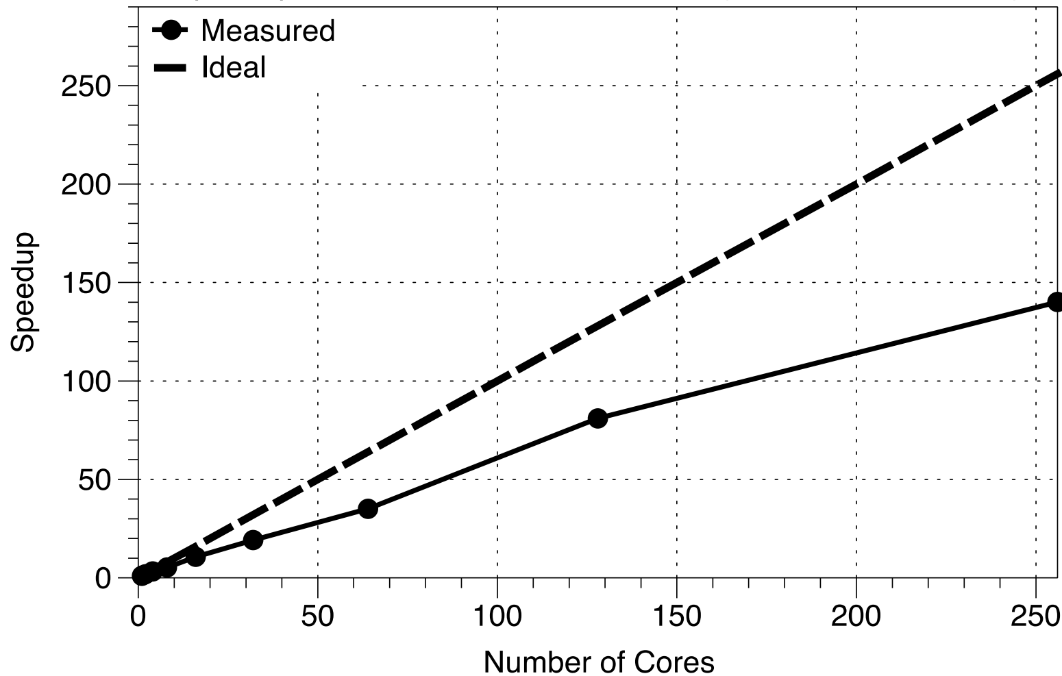
Speedup of CitcomS on TACC Lonestar (6.4 million unknowns)
