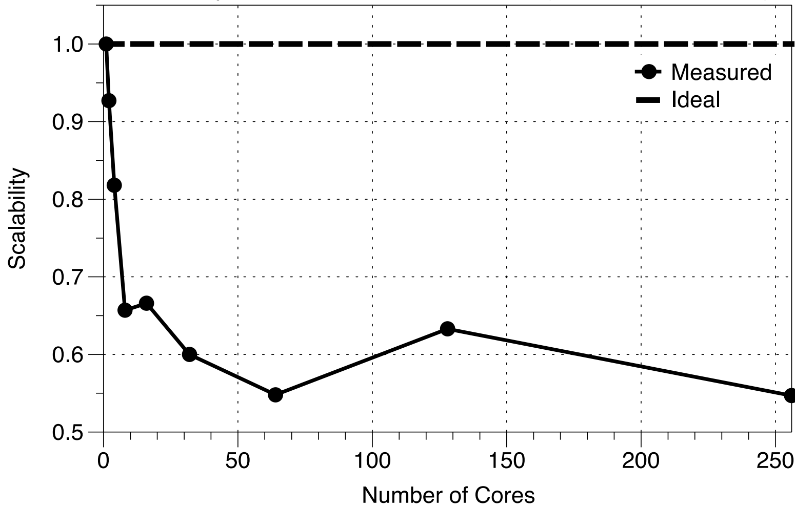
Scalability of CitcomS on TACC Lonestar (6.4 million unknowns)
