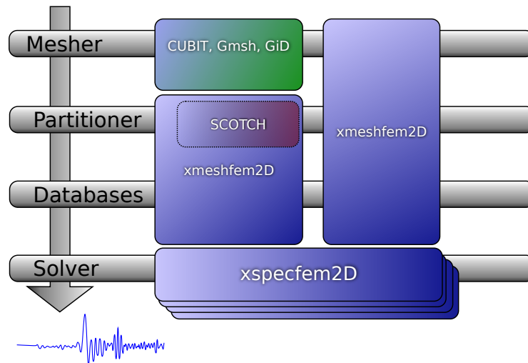
Figure 3.1: Schematic workflow for a SPECSEM2D simulation. The executable xmeshfem2D creates the GLL mesh points and assigns specific model parameters. The executable xspecfem2D solves the seismic wave propagation.
